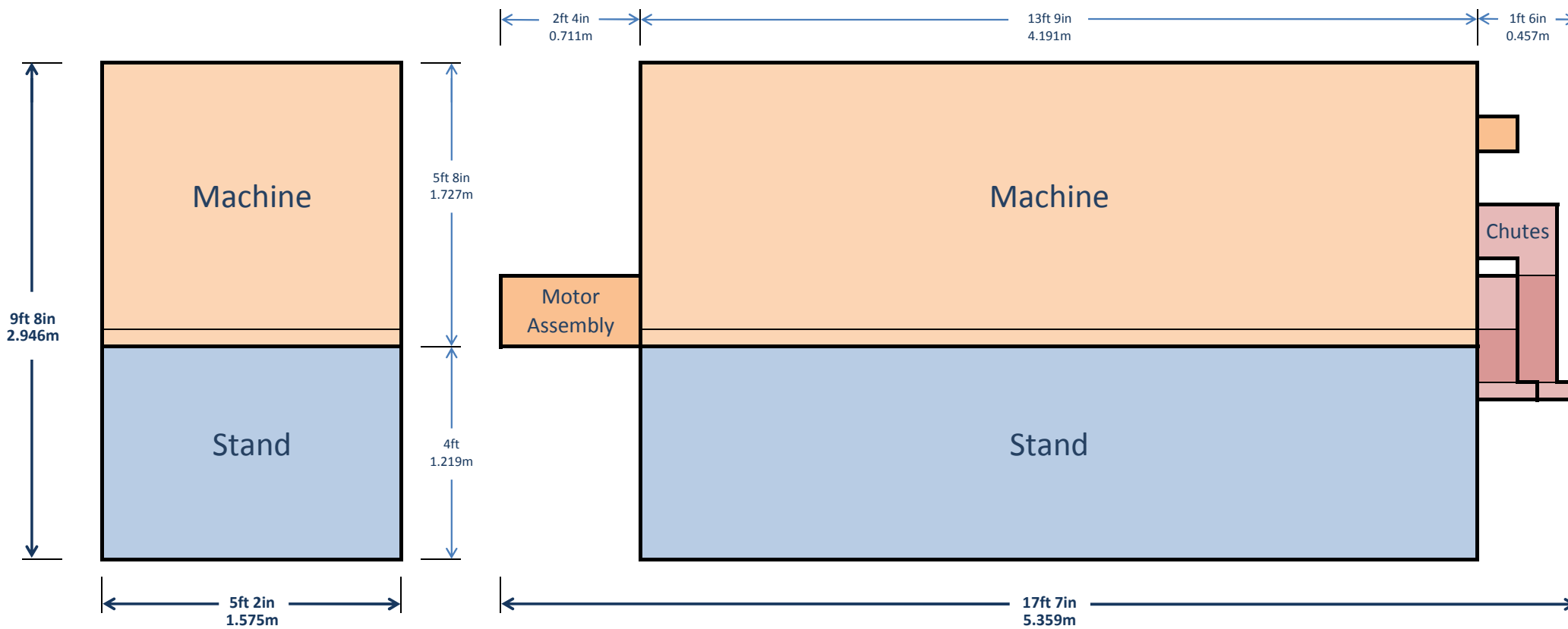
End View
